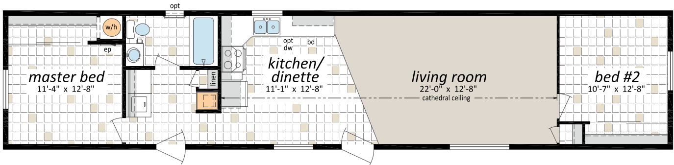
AS-2013, "The Amity" 14'x 66', 924 sq. ft.
